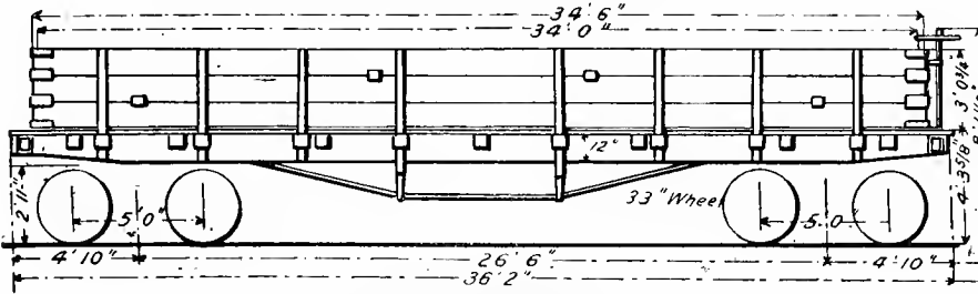
Fig. 65. Side Elevation.
